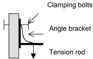
Figure 3 Example of test assembly
