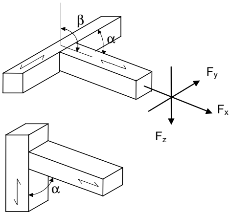
Arrangement and loading of timber members with end-grain to side-grain
