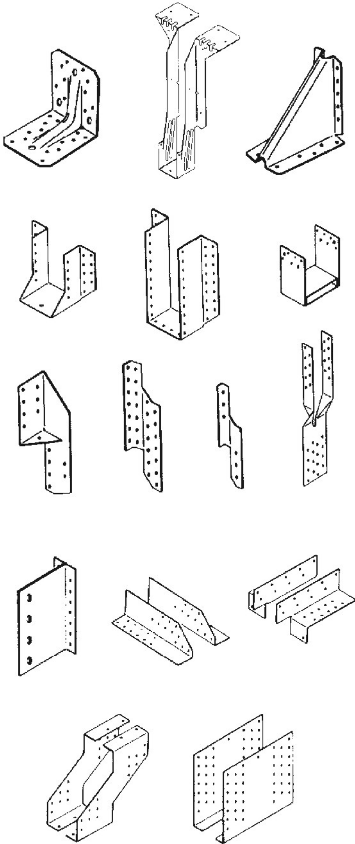
Figure 1 Examples of three-dimensional nailing plates
