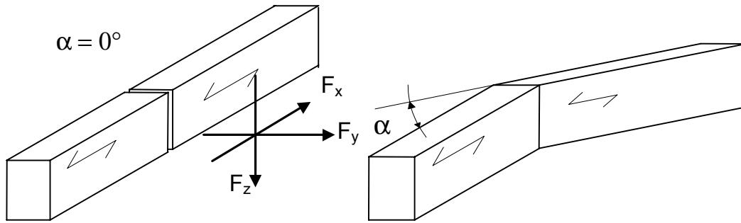
Arrangement and loading of timber members with end-grain to end-grain
