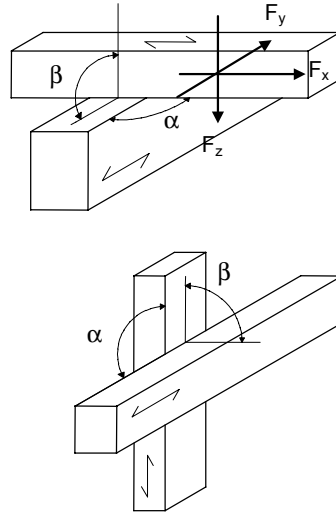
Arrangement and loading of timber members with side-grain to side-grain
